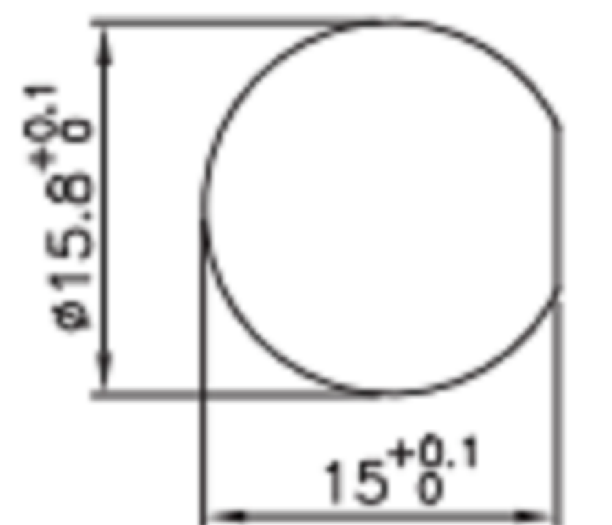
开孔尺寸 hole opening size
